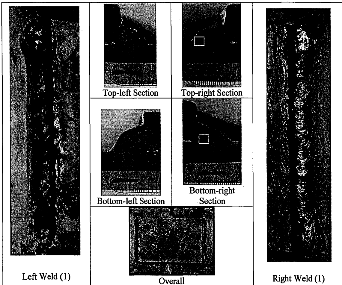
Figure 5.8: Specimen 36G-17HR
