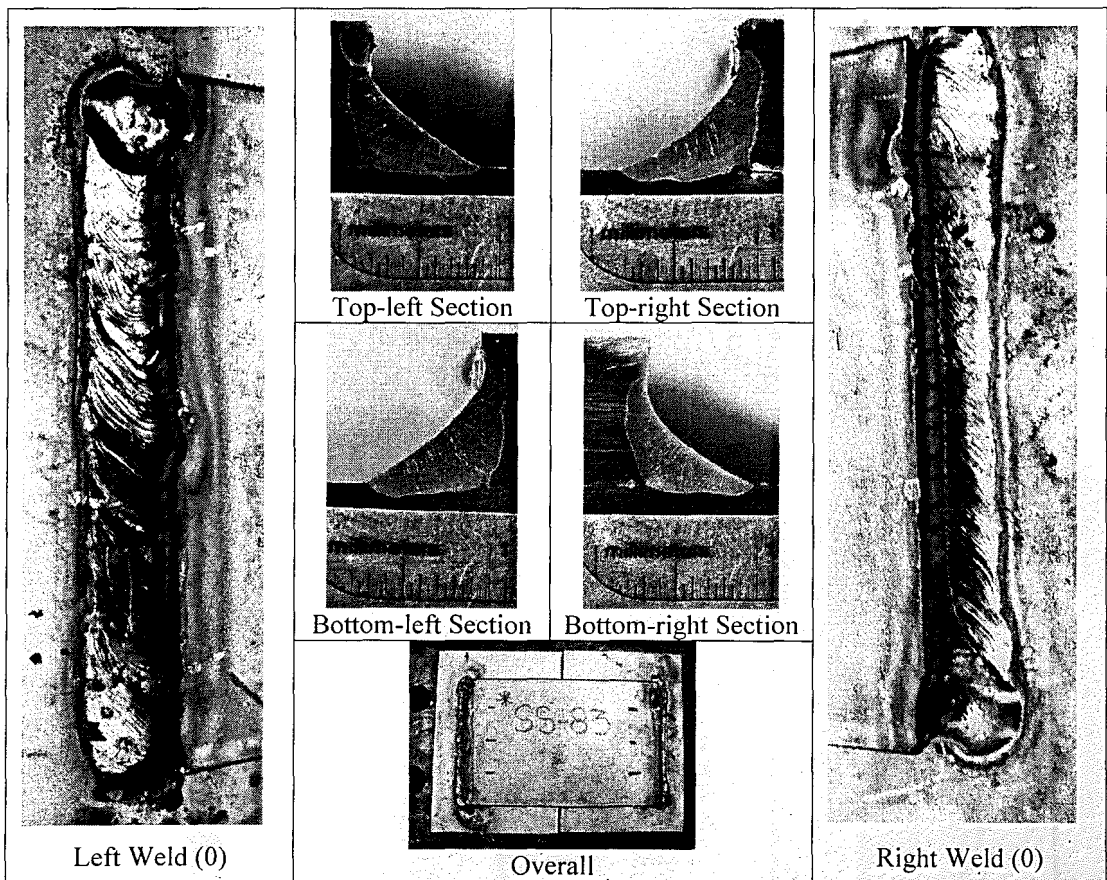
Figure 6.12: Specimen SS-83
