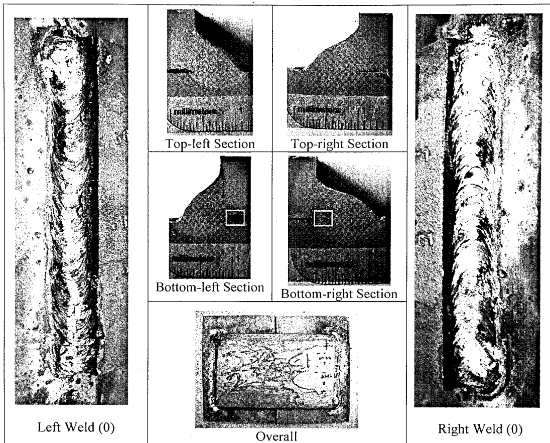
Figure 4.27: Specimen 36-C1
