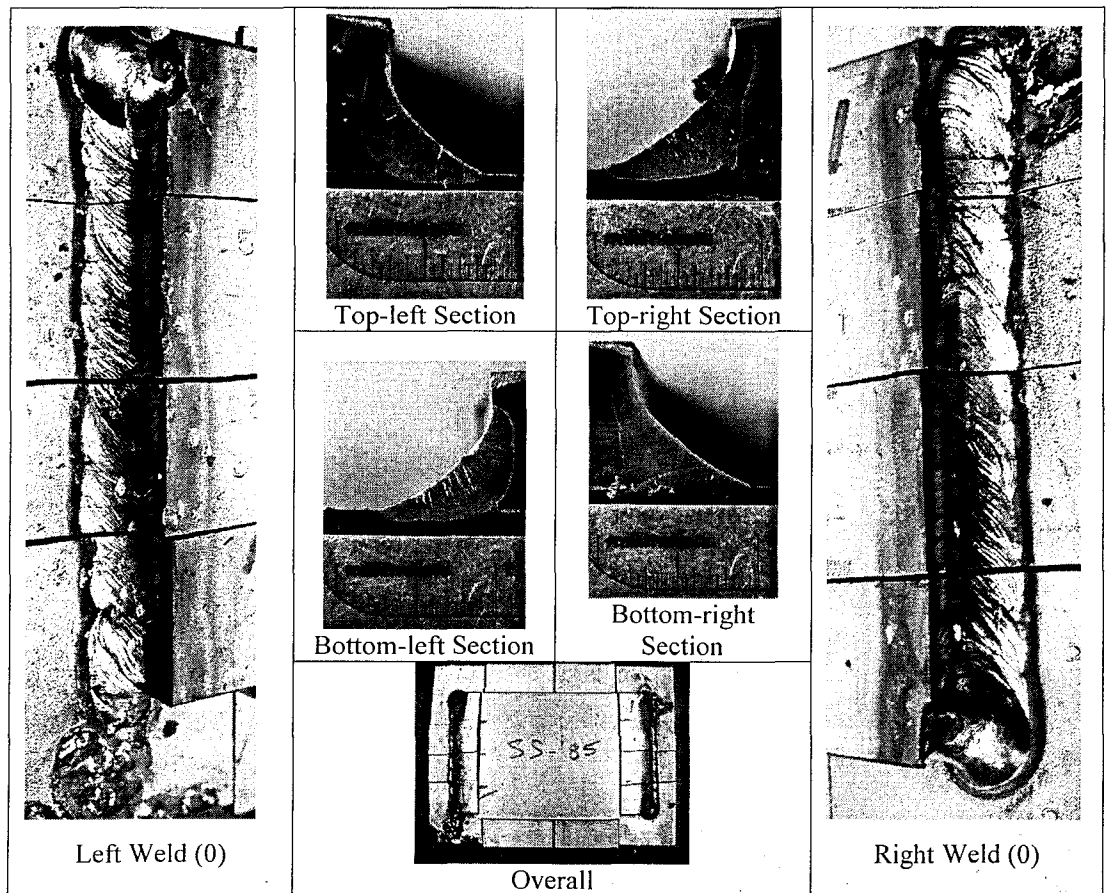
Figure 6.14: Specimen SS-85
