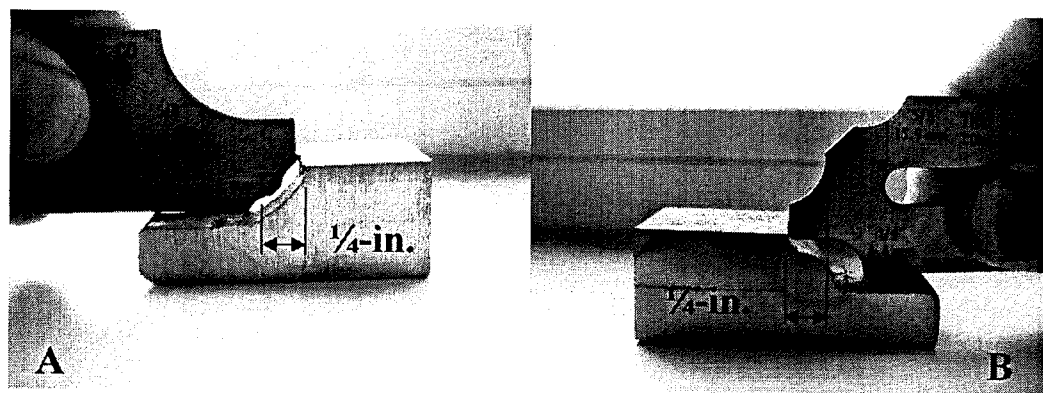
Figure 3.11: Fillet Weld Gage—Concave Measurement (A), Convex Measurement (B)
