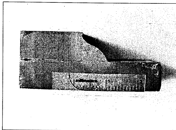
Figure 3.9: Polished A36 Cross Section
