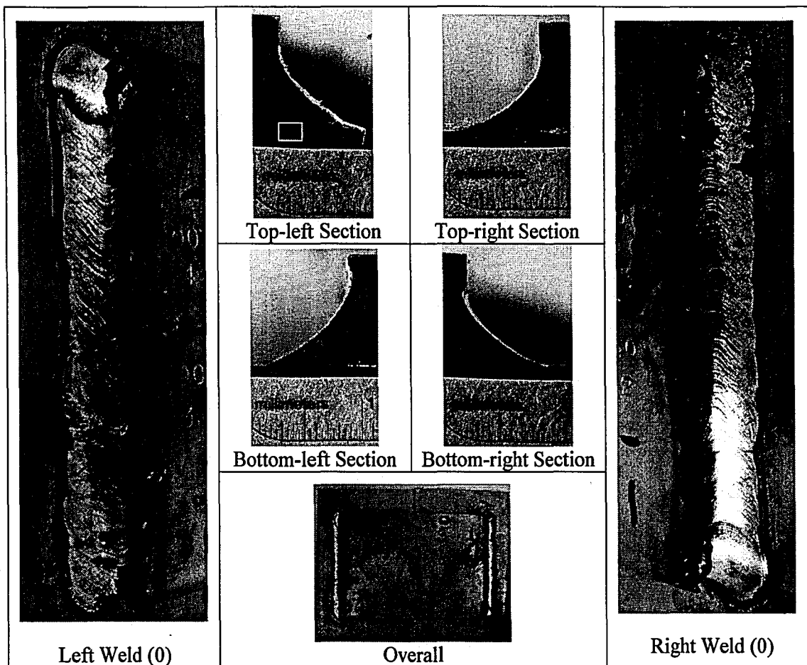
Figure 6.21: Specimen SS-90
