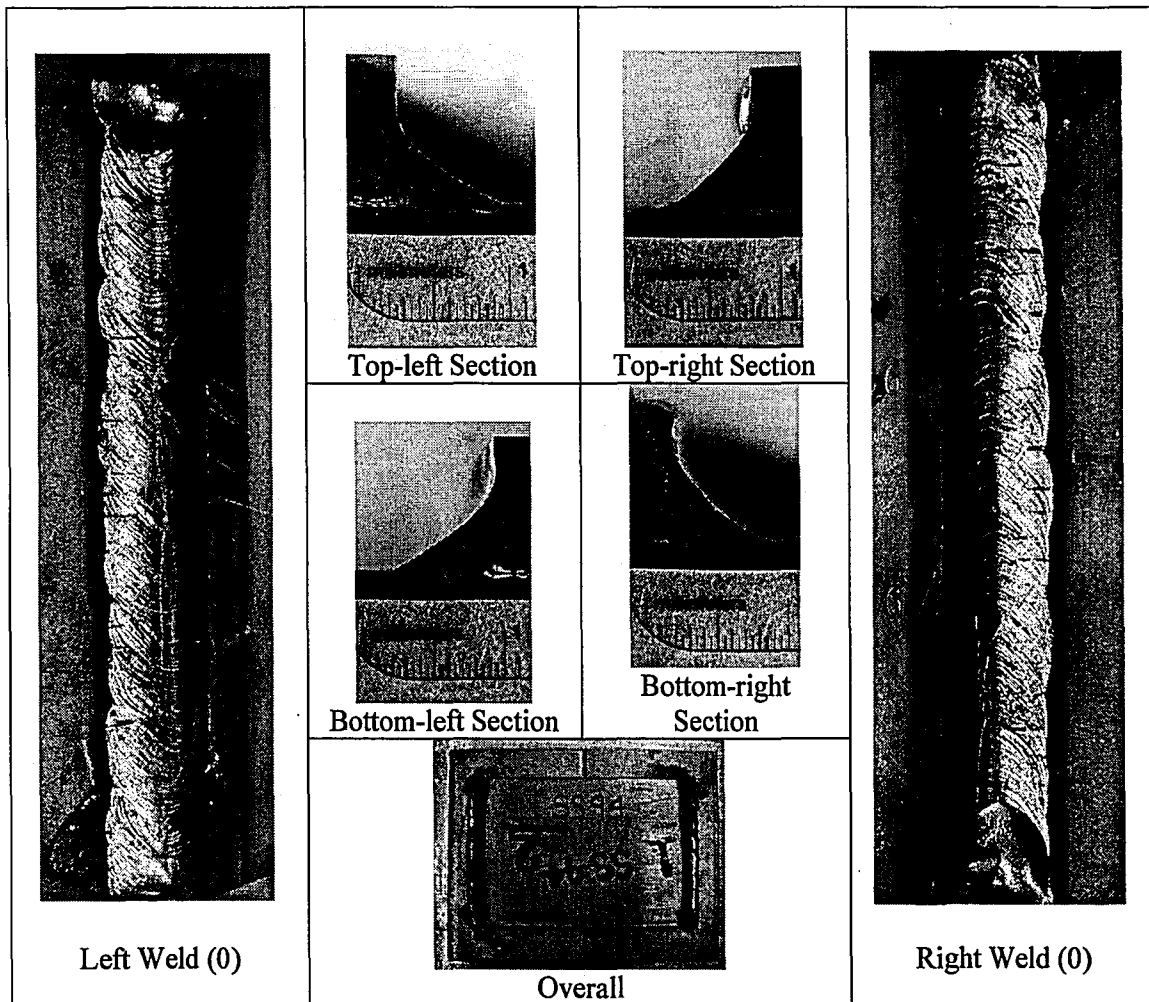
Figure 6.27: Specimen SS-94
