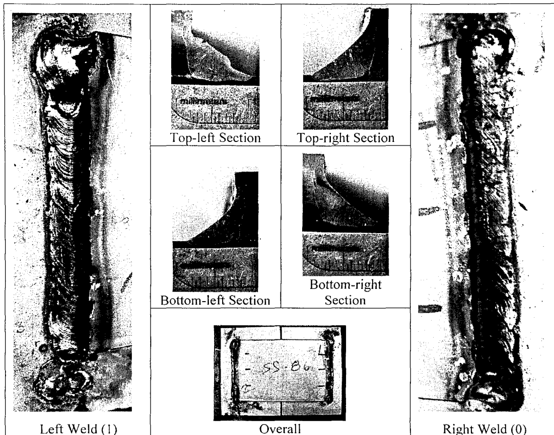
Figure 6.15: Specimen SS-86
