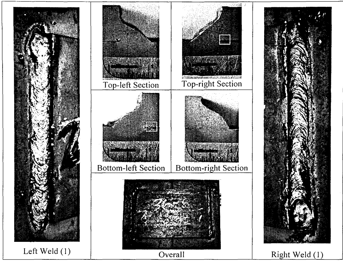
Figure 4.6: Specimen 36-6
