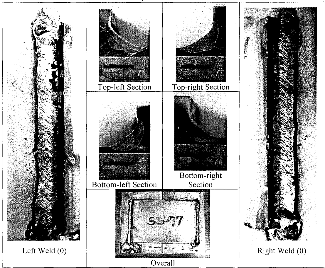
Figure 6.8: Specimen SS-77
