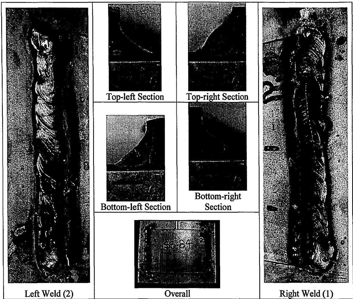
Figure 6.13: Specimen SS-84
