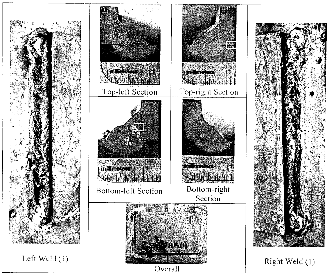
Figure 4.22: Specimen 36-17HR(1)
