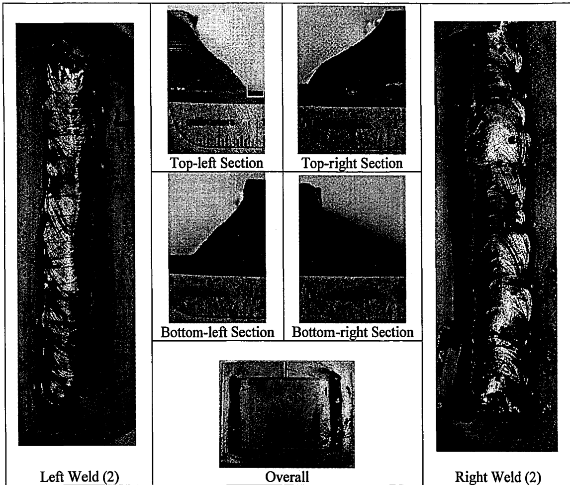
Figure 6.31: Specimen SS-(1/4)35
