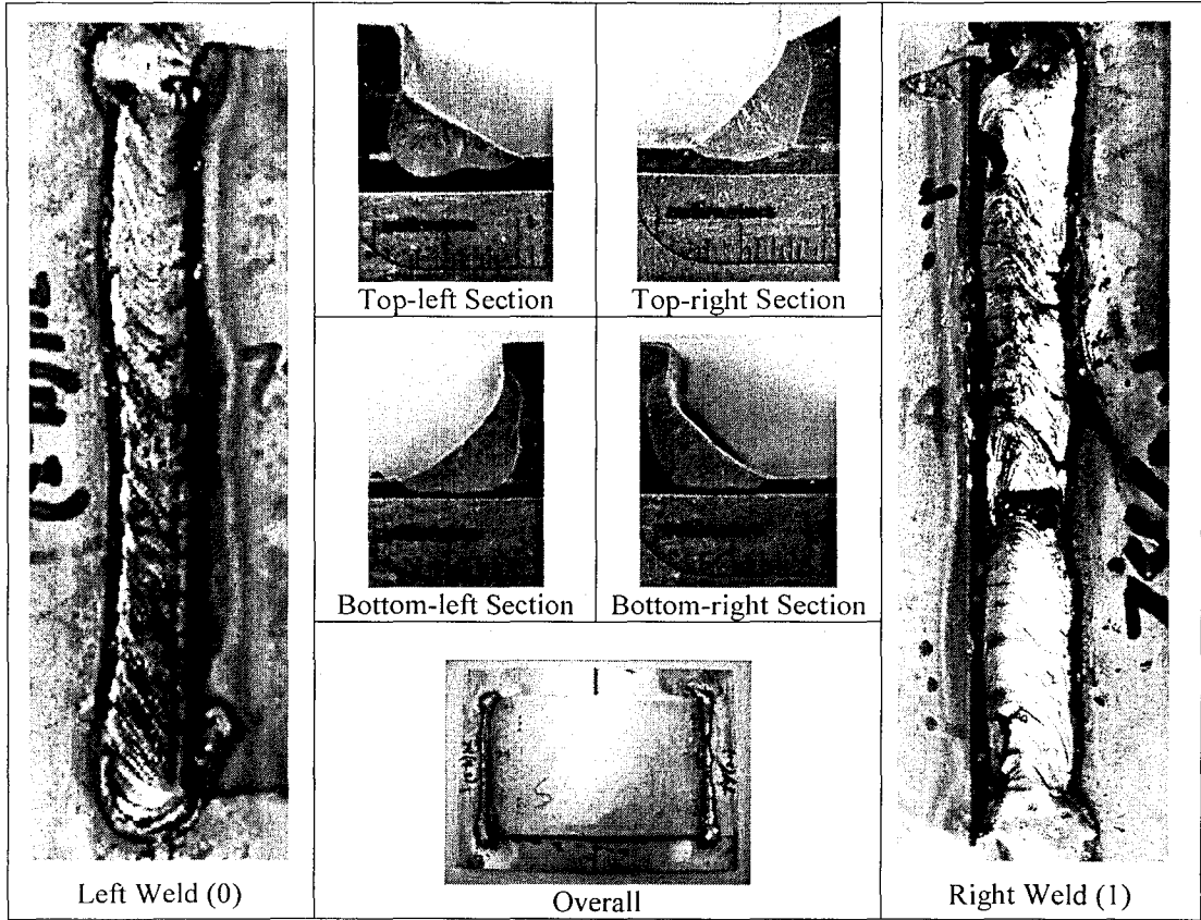
Figure 6.4: Specimen SS-74
