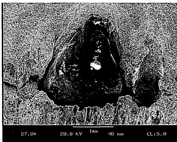
Figure 8.18: SEM Image (27.8x) of Large Inclusion—T-3
