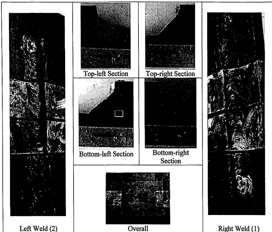
Figure 4.14: Specimen 36-14
