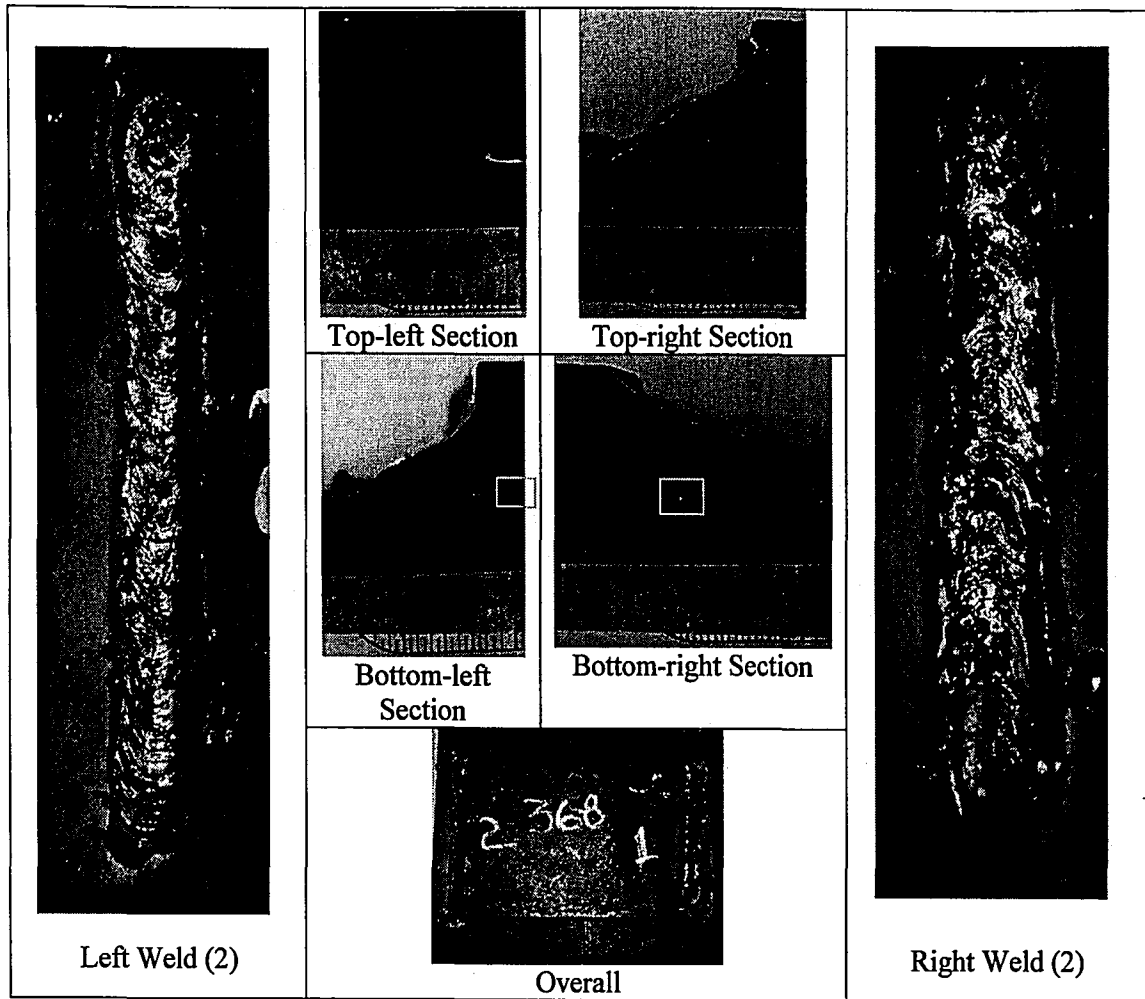
Figure 4.11: Specimen 36-8
