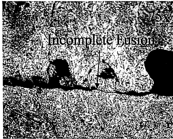
Figure 4.12: Incomplete Fusion in Specimen 36-8, Bottom-right section
