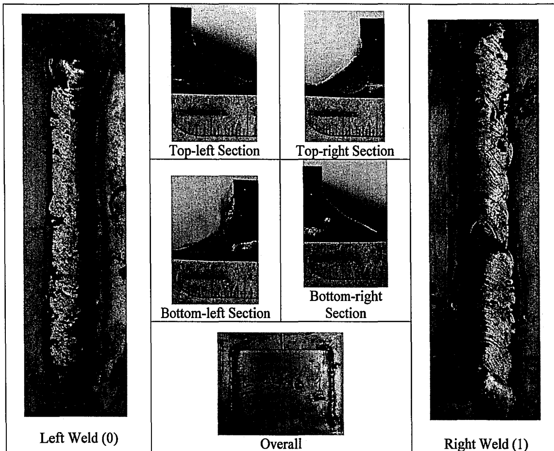
Figure 6.29: Specimen SS-96
