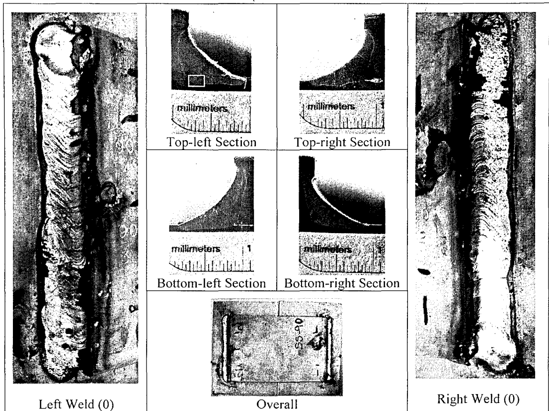
Figure 6.21: Specimen SS-90
